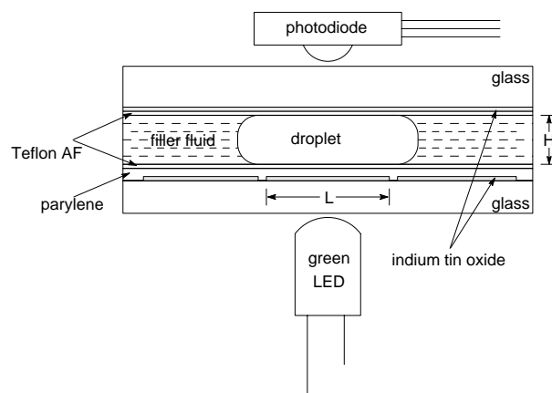
Fig 1 - Schematic of device (vertical cross section)
