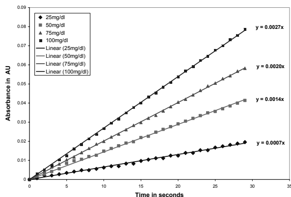
Fig 2 - Absorbance vs Time (DF = 2)
