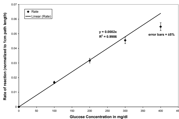
Fig 5 - Rate vs Glucose concentration (Linear Range)
