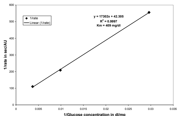
Fig 6 - Lineweaver-Burke plots
