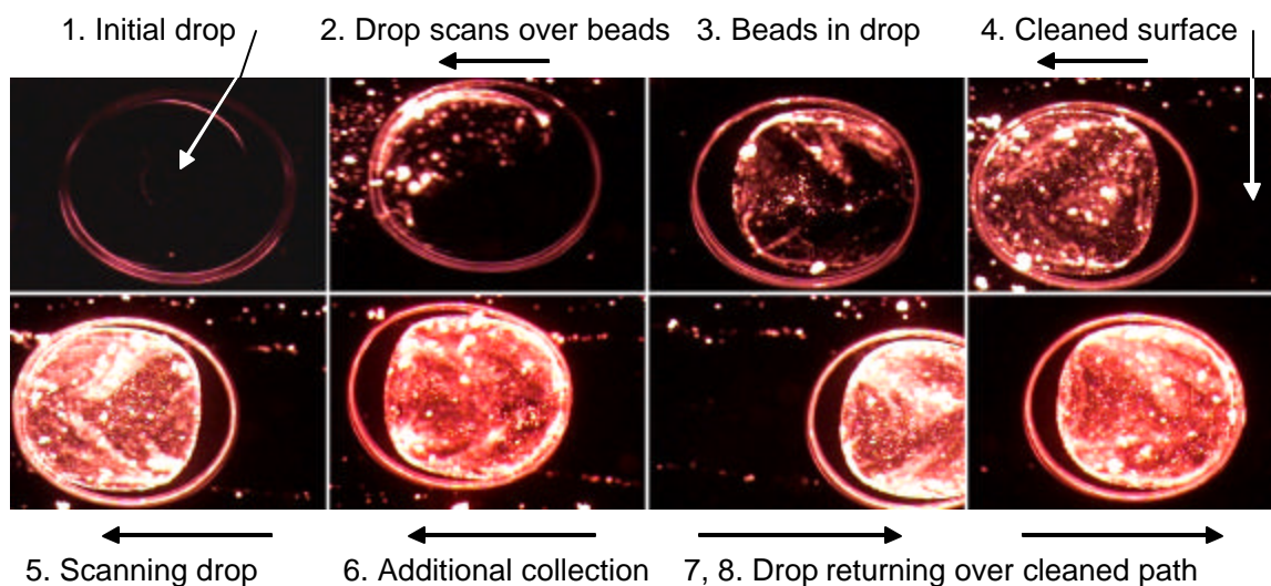
Figure 5. Demonstration of the scanning-droplet particle collection process. Arrows indicate the direction of droplet scan, and the frame numbers show the time sequence. It can be seen that the deposited 1µm beads on the surface are picked up, leaving a cleaned swath behind the droplet. No beads are re-deposited once the scan direction is reversed.
