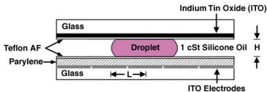
Figure 1 - Side view of the electrowetting chip showing the material layers
